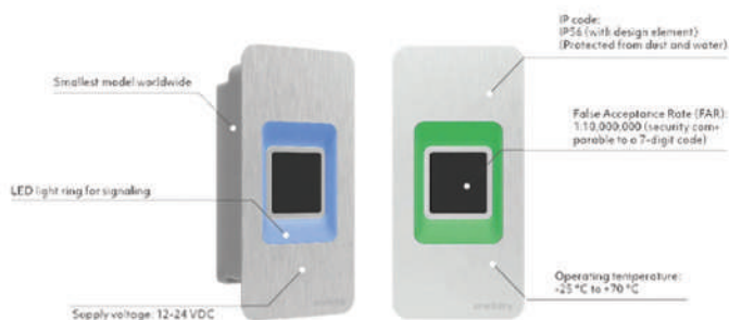
ekey dLine fingerprint scanner
